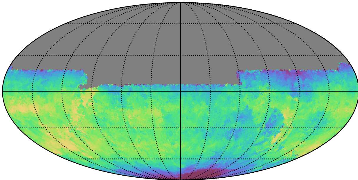
ddf_half_v3.4_10yrs All sky u band: Median fiveSigmaDepth
