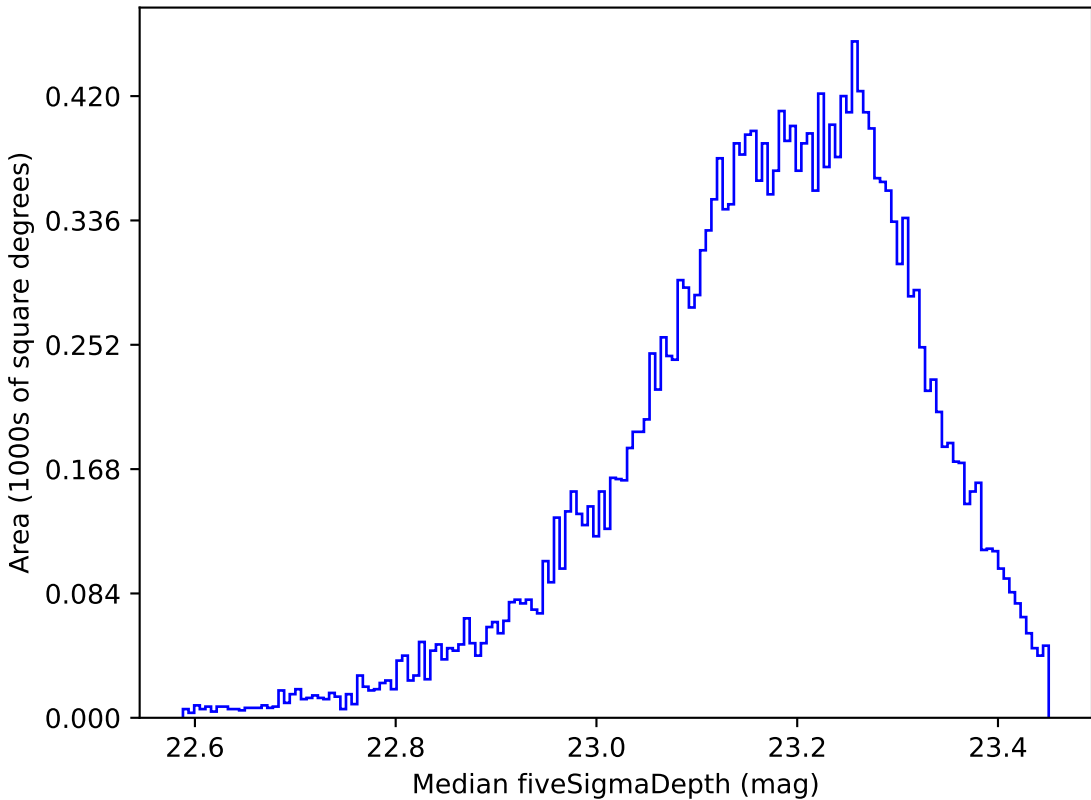
ddf_half_v3.4_10yrs All sky u band: Median fiveSigmaDepth
