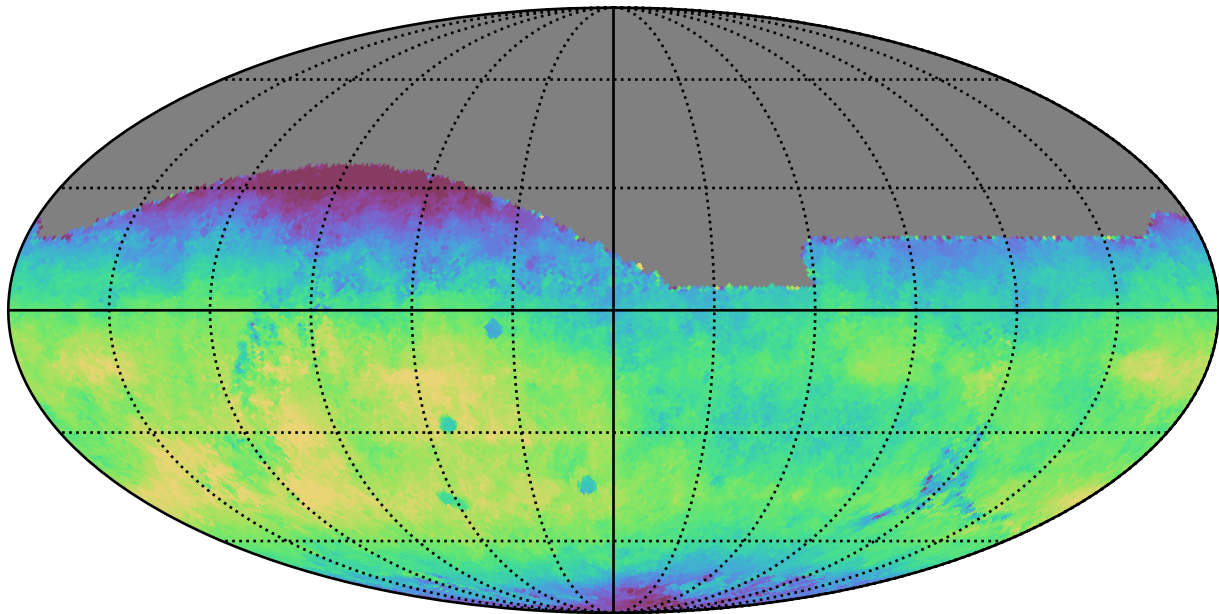
ddf_half_v3.4_10yrs All sky r band: Median fiveSigmaDepth
