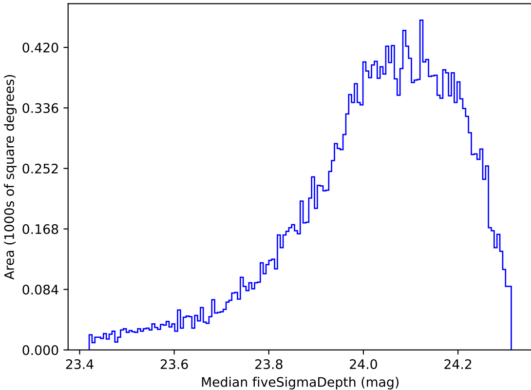
ddf_half_v3.4_10yrs All sky r band: Median fiveSigmaDepth
