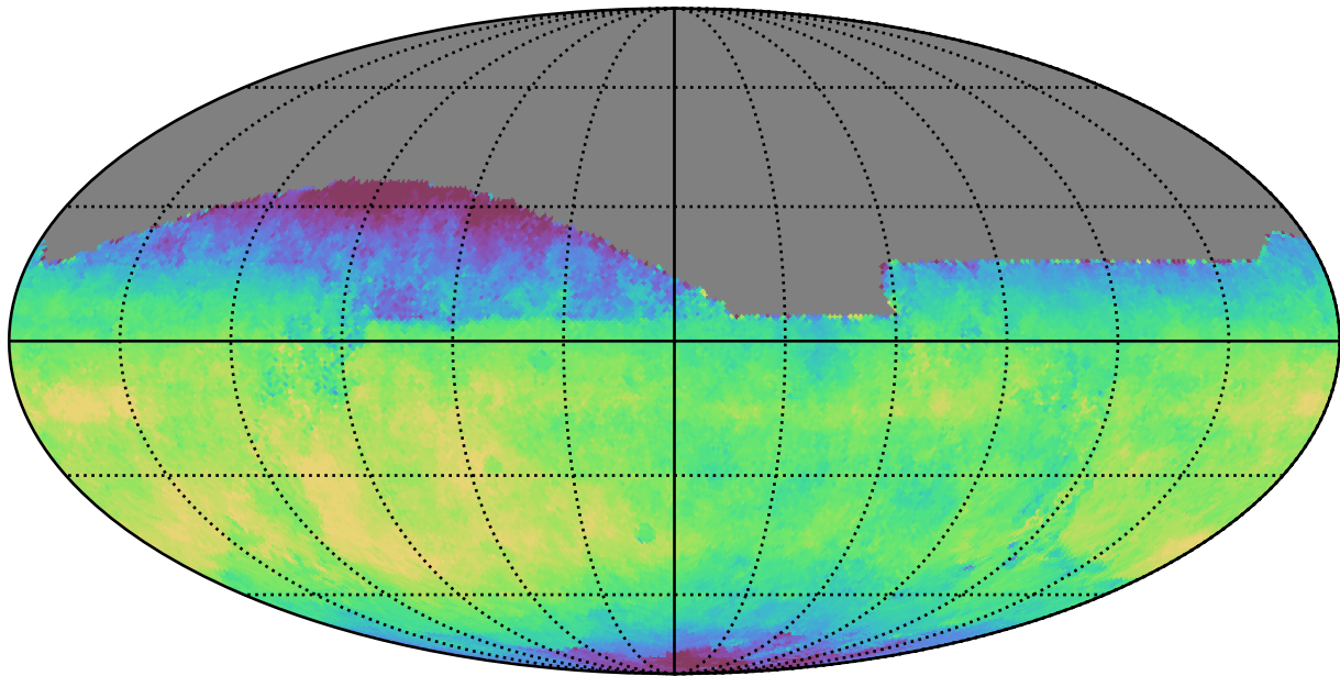
ddf_half_v3.4_10yrs All sky i band: Median fiveSigmaDepth
