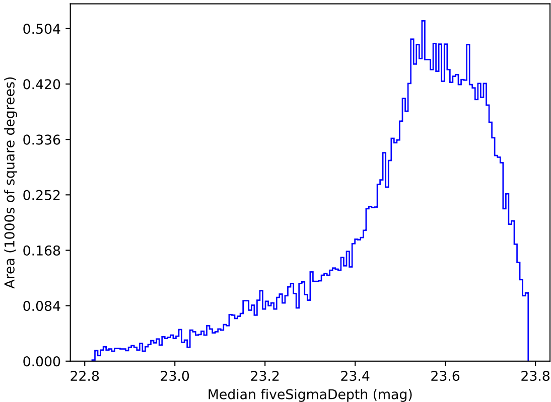
ddf_half_v3.4_10yrs All sky i band: Median fiveSigmaDepth
