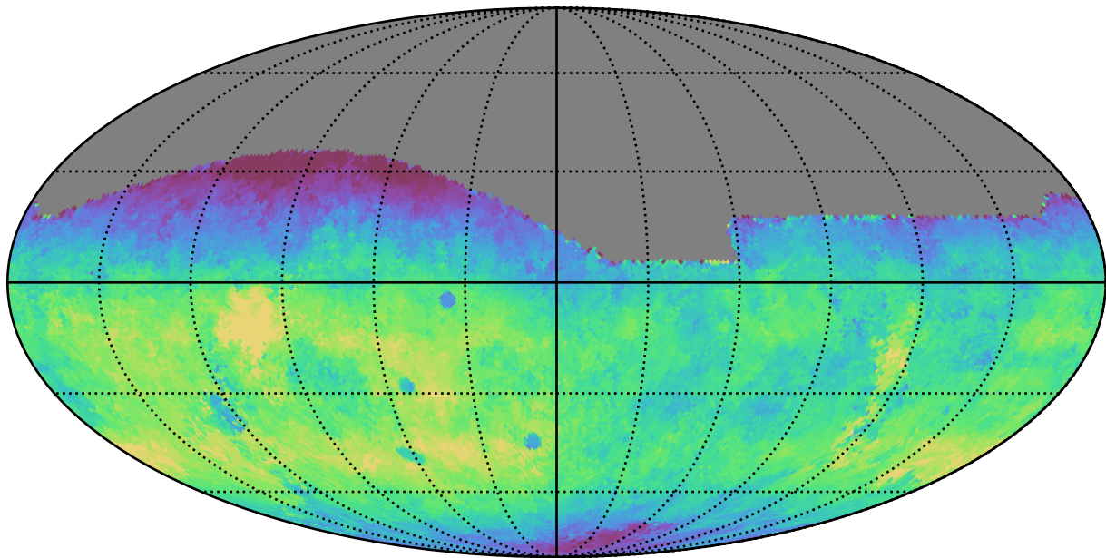
ddf_half_v3.4_10yrs All sky g band: Median fiveSigmaDepth
