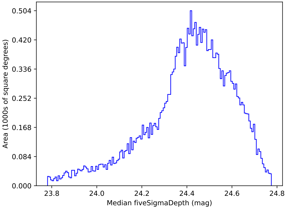
ddf_half_v3.4_10yrs All sky g band: Median fiveSigmaDepth
