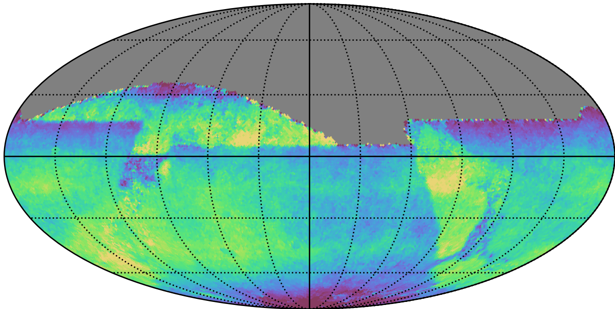
ddf_half_v3.4_10yrs All sky all bands: Median fiveSigmaDepth
