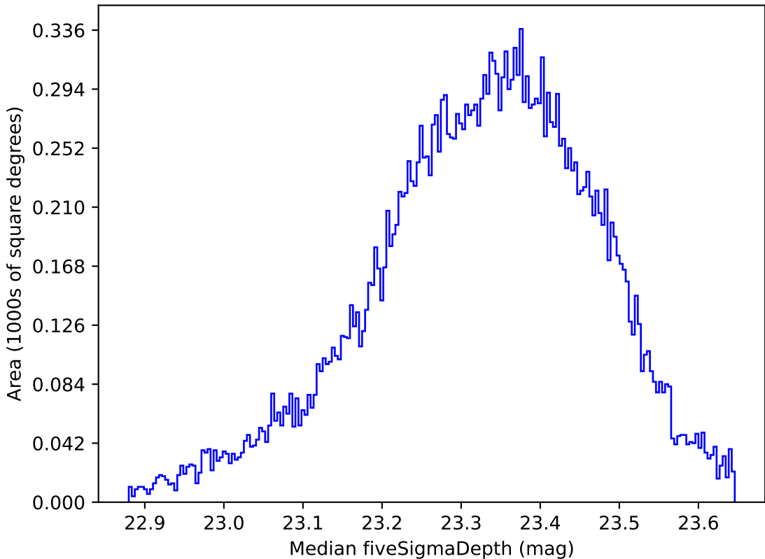
ddf_half_v3.4_10yrs All sky all bands: Median fiveSigmaDepth
