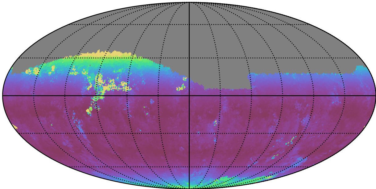
ddf_half_v3.4_10yrs Yr 1 z band: Median airmass
