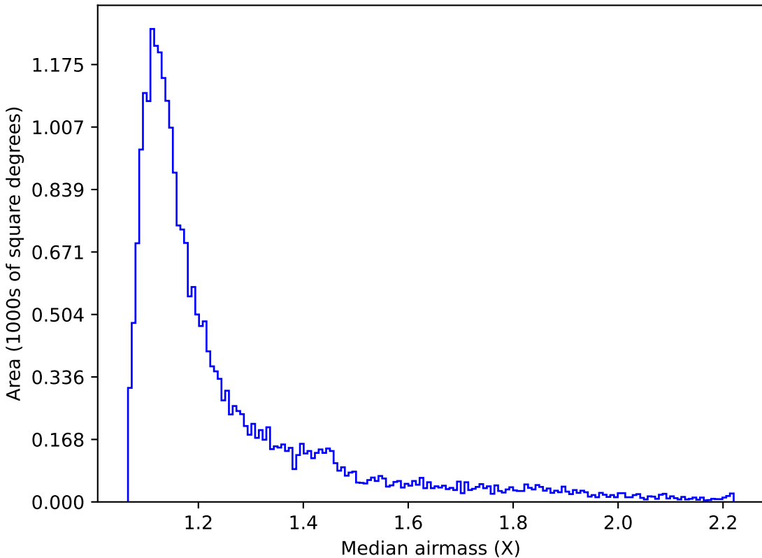
ddf_half_v3.4_10yrs Yr 1 z band: Median airmass
