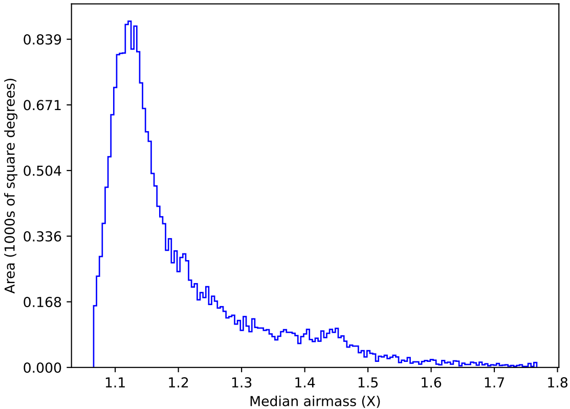
ddf_half_v3.4_10yrs Yr 1 y band: Median airmass
