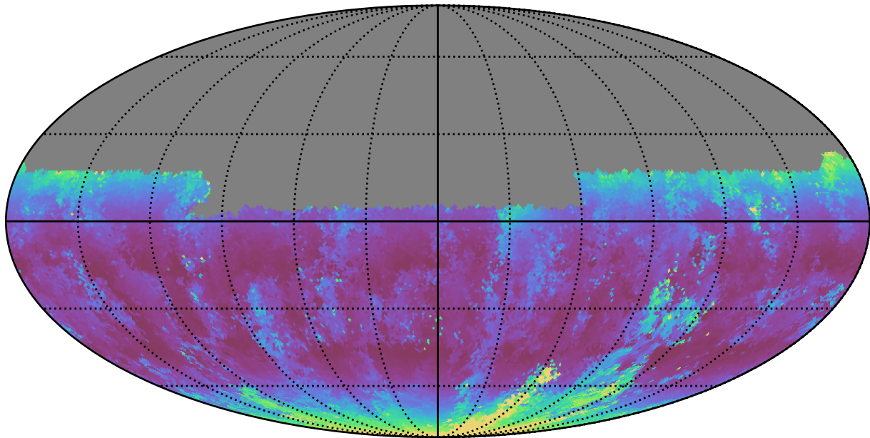
ddf_half_v3.4_10yrs Yr 1 u band: Median airmass
