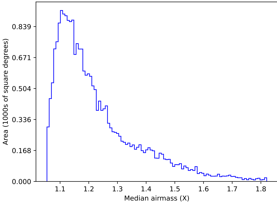
ddf_half_v3.4_10yrs Yr 1 u band: Median airmass
