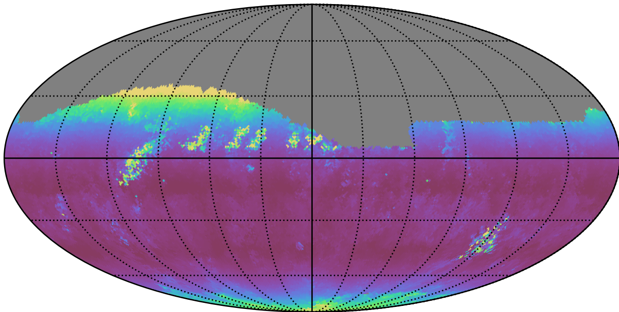
ddf_half_v3.4_10yrs Yr 1 r band: Median airmass
