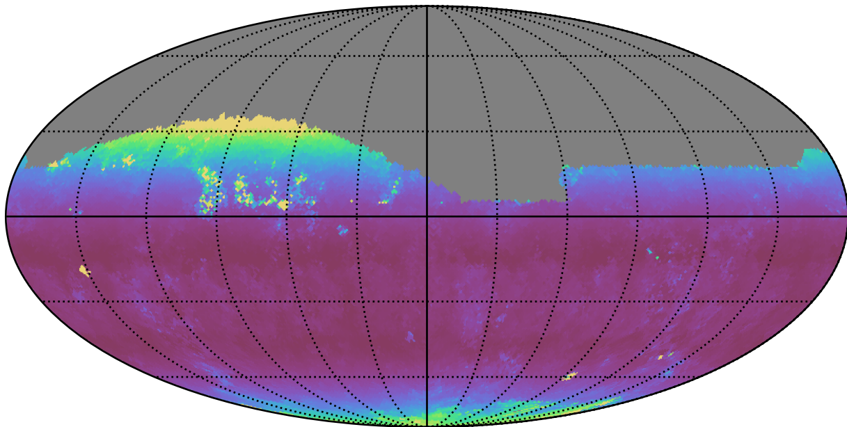
ddf_half_v3.4_10yrs Yr 1 i band: Median airmass
