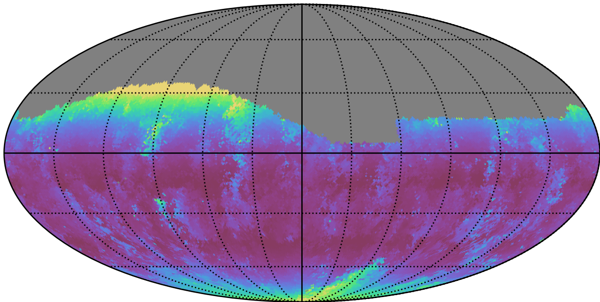
ddf_half_v3.4_10yrs Yr 1 g band: Median airmass
