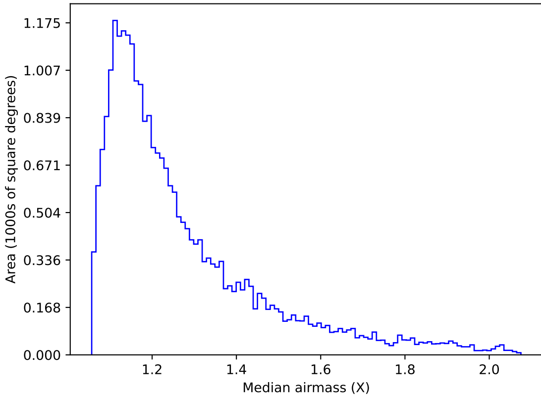
ddf_half_v3.4_10yrs Yr 1 g band: Median airmass
