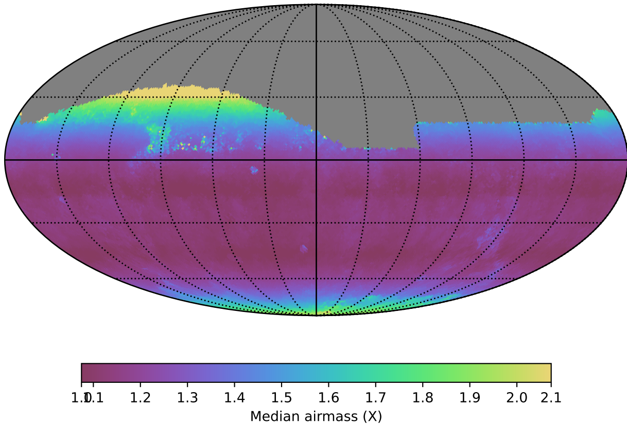
ddf_half_v3.4_10yrs Yr 1 all bands: Median airmass
