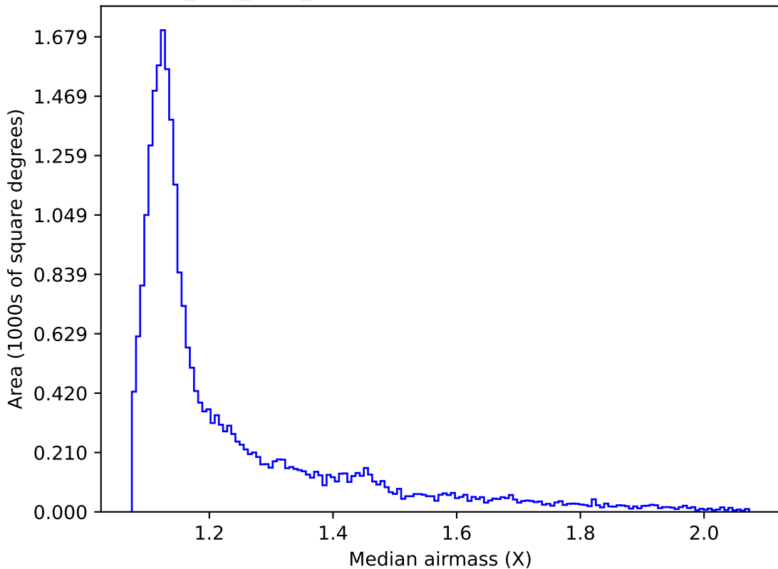
ddf_half_v3.4_10yrs Yr 1 all bands: Median airmass
