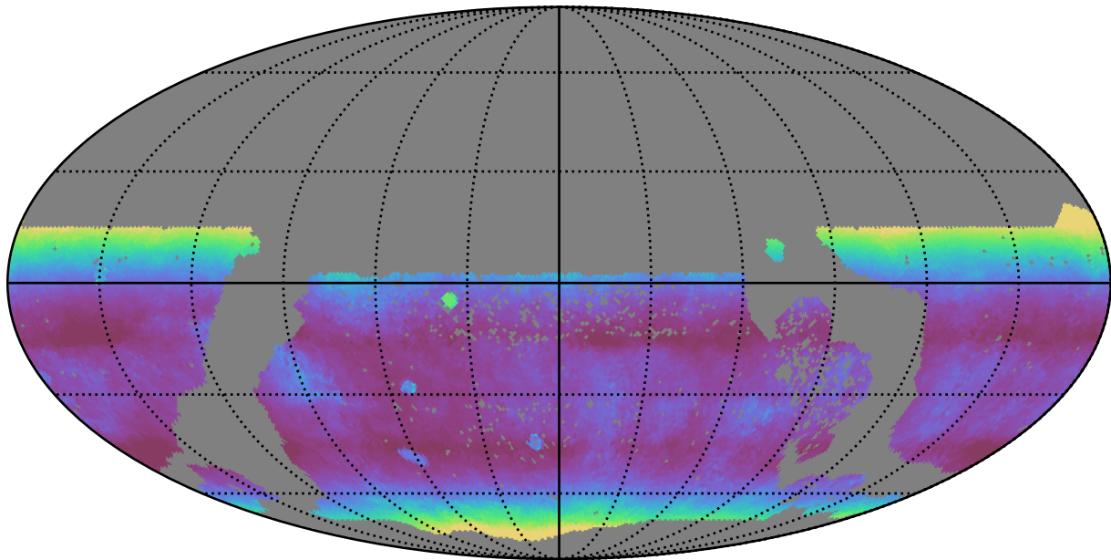
ddf_half_v3.4_10yrs WFD z band: Median airmass
