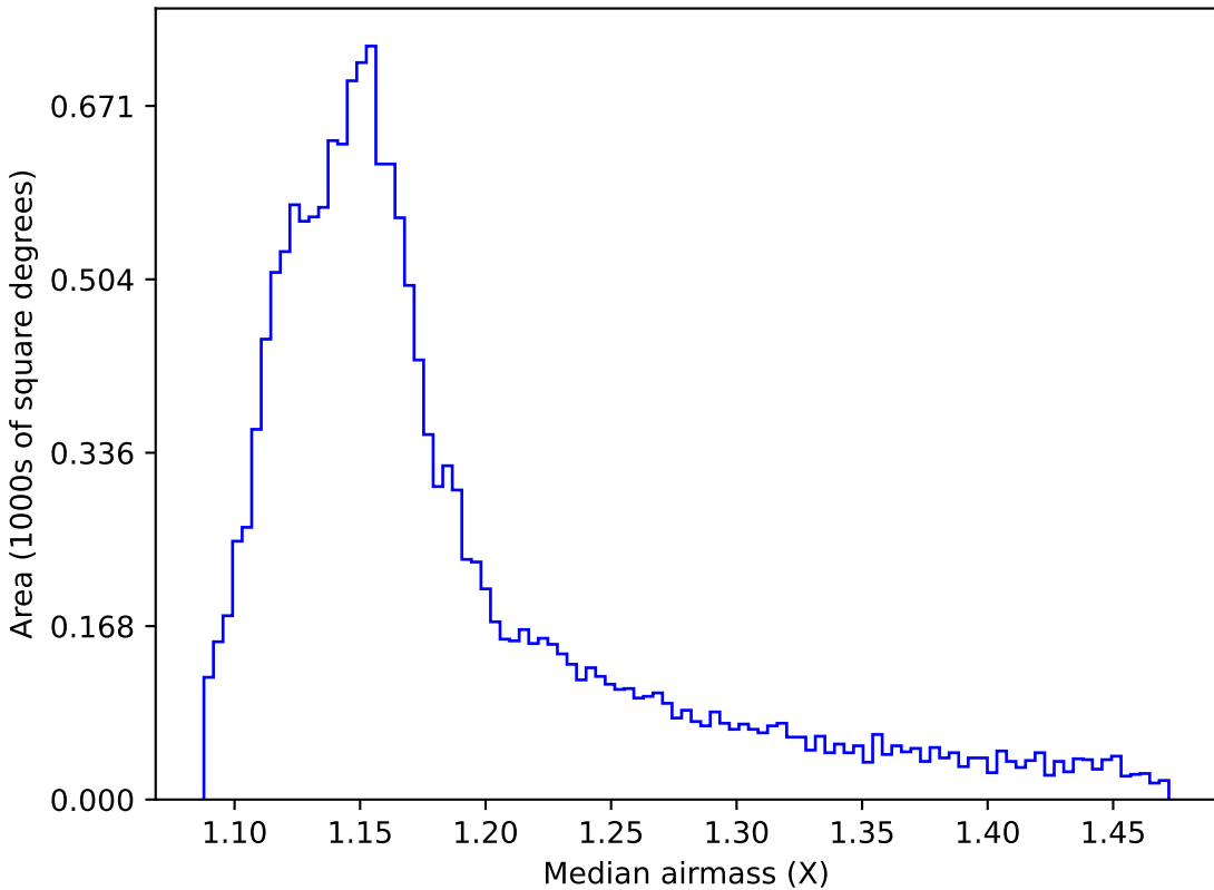
ddf_half_v3.4_10yrs WFD z band: Median airmass
