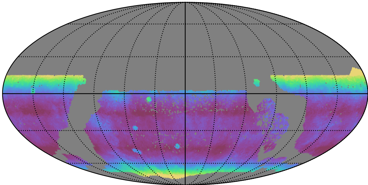
ddf_half_v3.4_10yrs WFD y band: Median airmass
