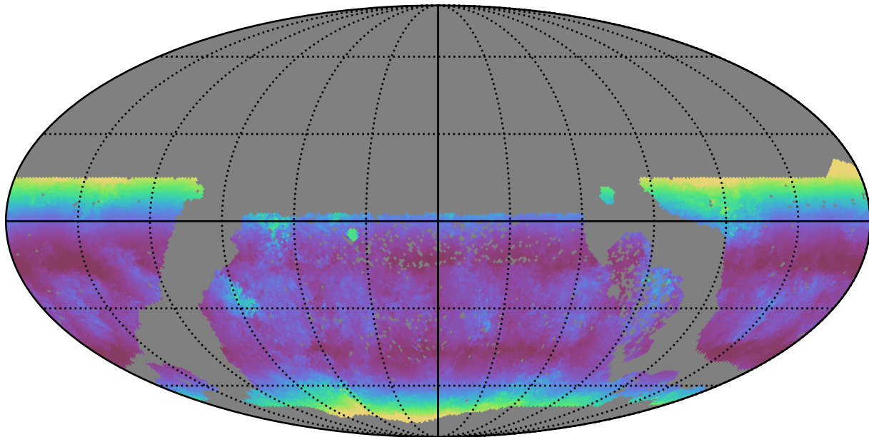
ddf_half_v3.4_10yrs WFD u band: Median airmass
