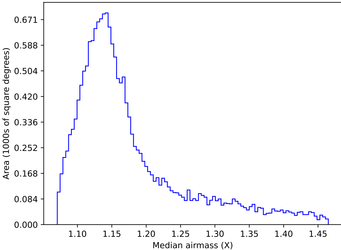
ddf_half_v3.4_10yrs WFD u band: Median airmass
