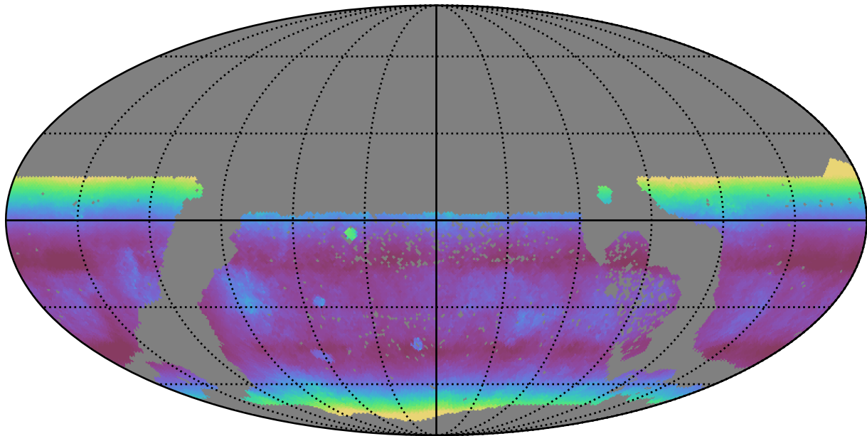
ddf_half_v3.4_10yrs WFD r band: Median airmass
