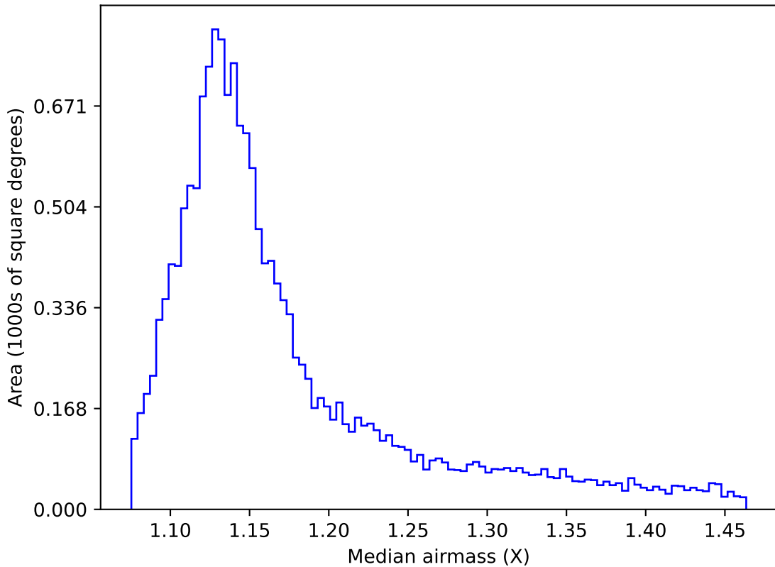
ddf_half_v3.4_10yrs WFD r band: Median airmass
