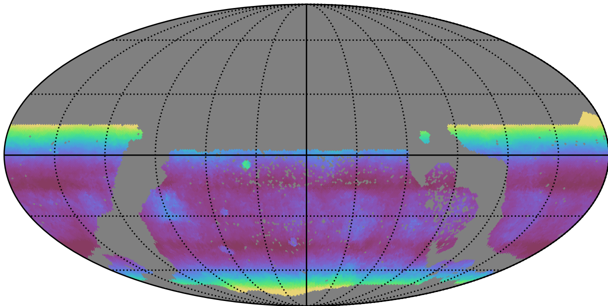
ddf_half_v3.4_10yrs WFD i band: Median airmass
