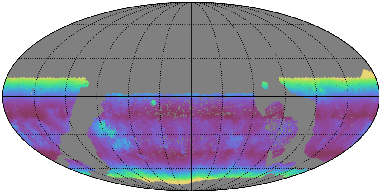
ddf_half_v3.4_10yrs WFD g band: Median airmass
