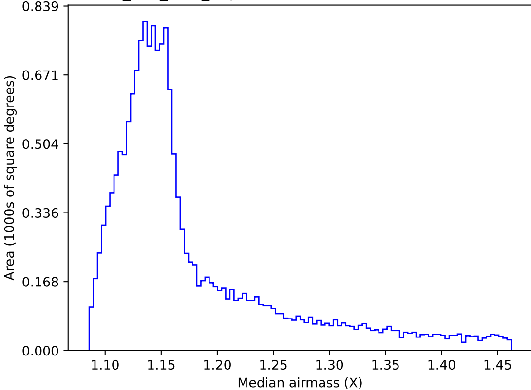
ddf_half_v3.4_10yrs WFD all bands: Median airmass
