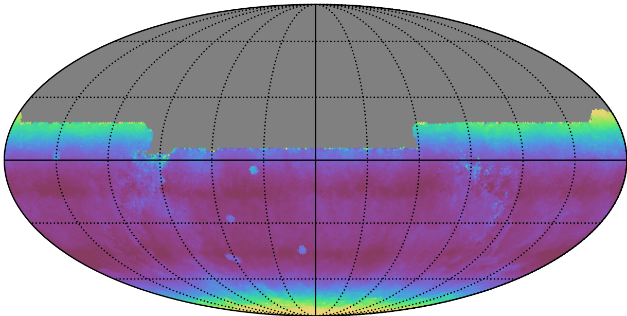
ddf_half_v3.4_10yrs All sky y band: Median airmass
