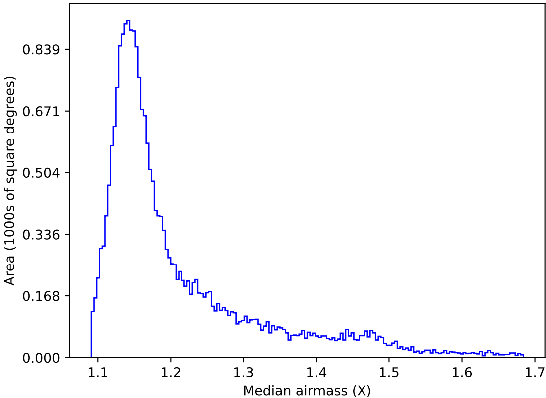
ddf_half_v3.4_10yrs All sky y band: Median airmass
