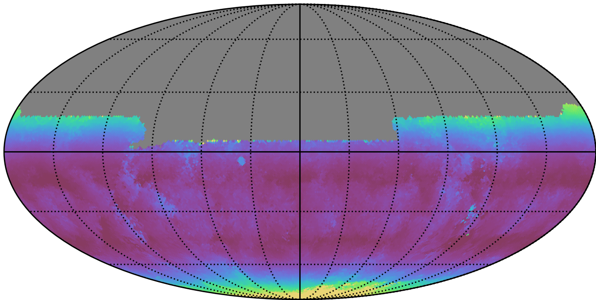
ddf_half_v3.4_10yrs All sky u band: Median airmass
