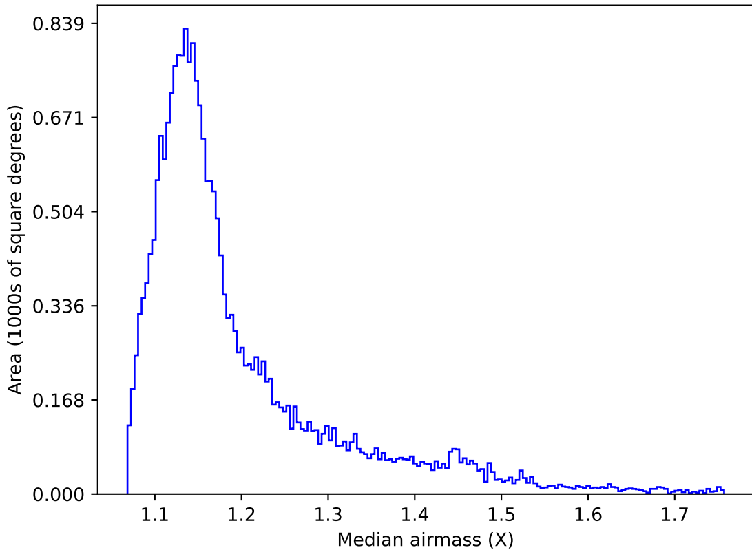
ddf_half_v3.4_10yrs All sky u band: Median airmass
