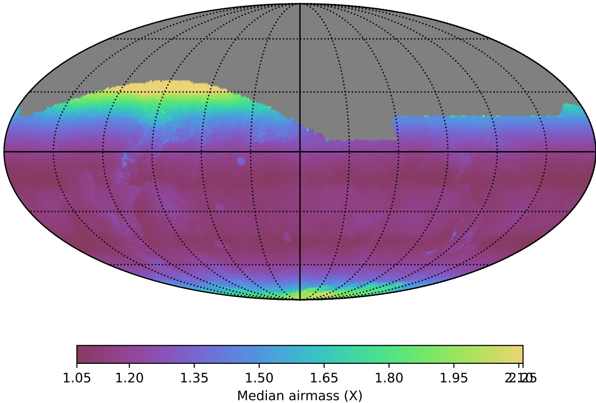
ddf_half_v3.4_10yrs All sky r band: Median airmass
