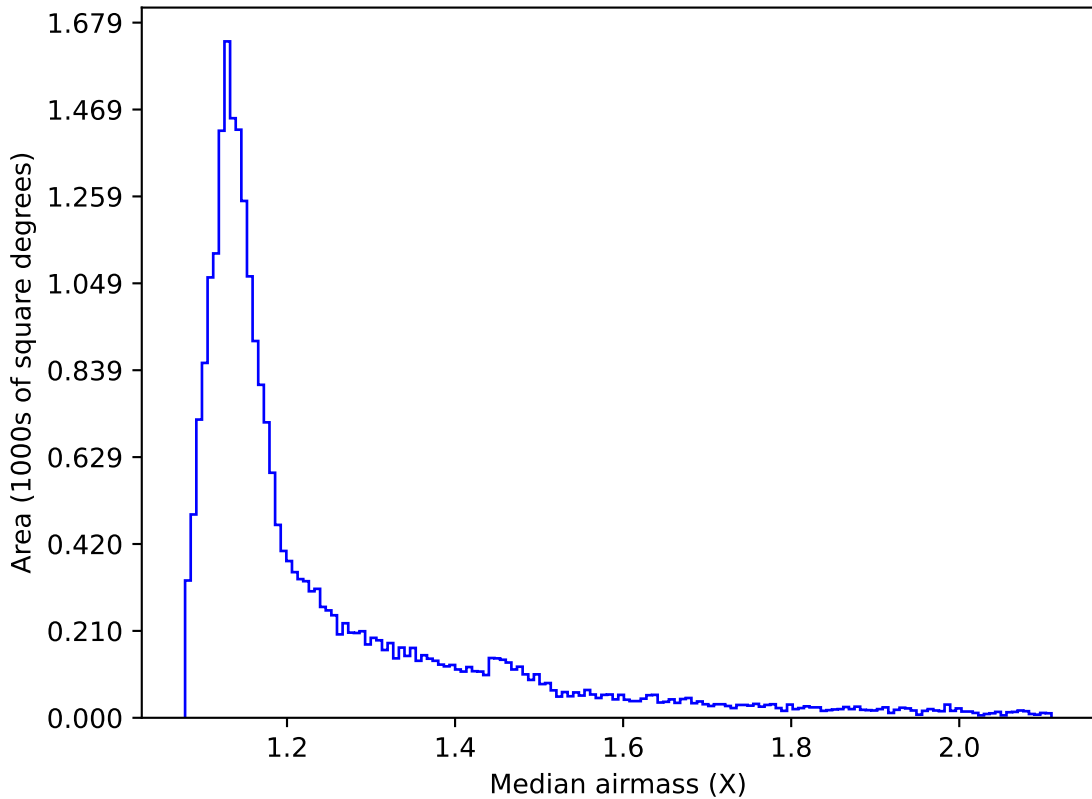
ddf_half_v3.4_10yrs All sky r band: Median airmass
