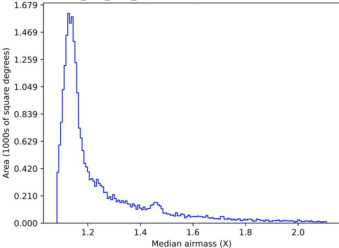
ddf_half_v3.4_10yrs All sky i band: Median airmass
