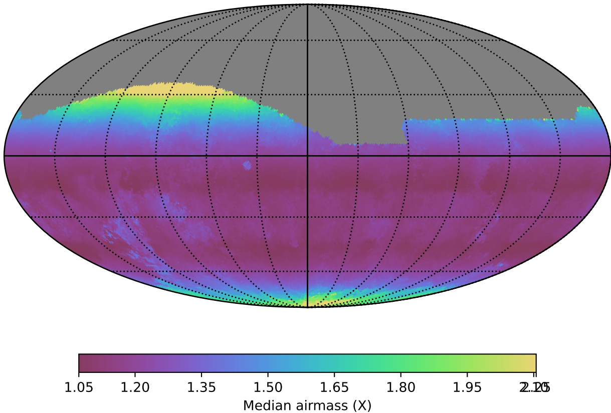
ddf_half_v3.4_10yrs All sky g band: Median airmass
