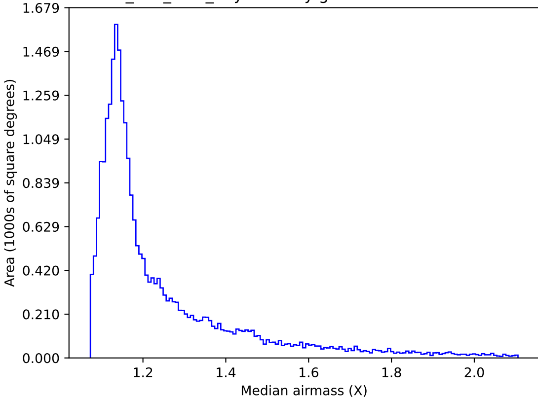
ddf_half_v3.4_10yrs All sky g band: Median airmass
