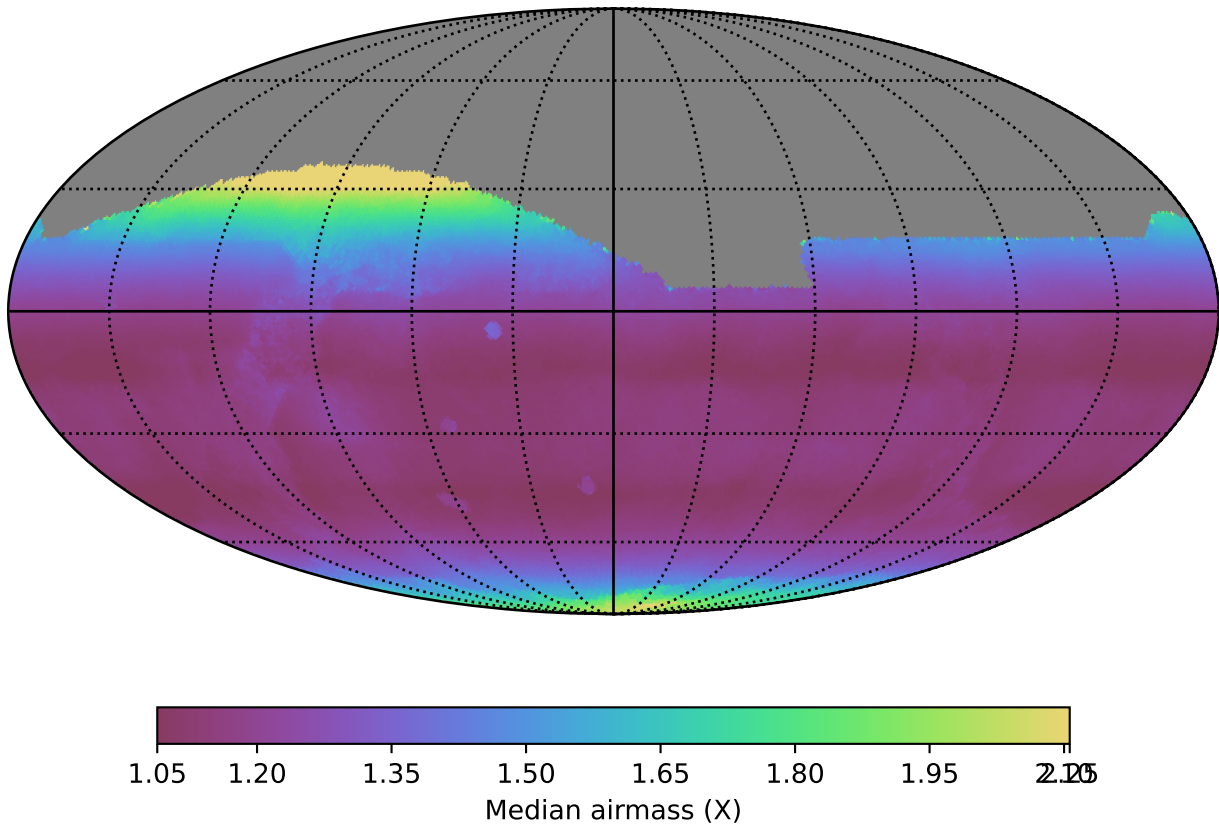
ddf_half_v3.4_10yrs All sky all bands: Median airmass
