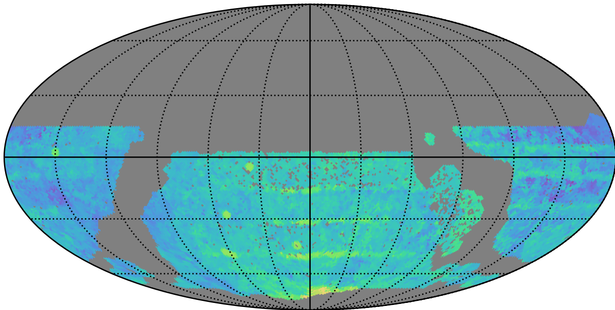
ddf_half_v3.4_10yrs WFD z band: Median Season Length
