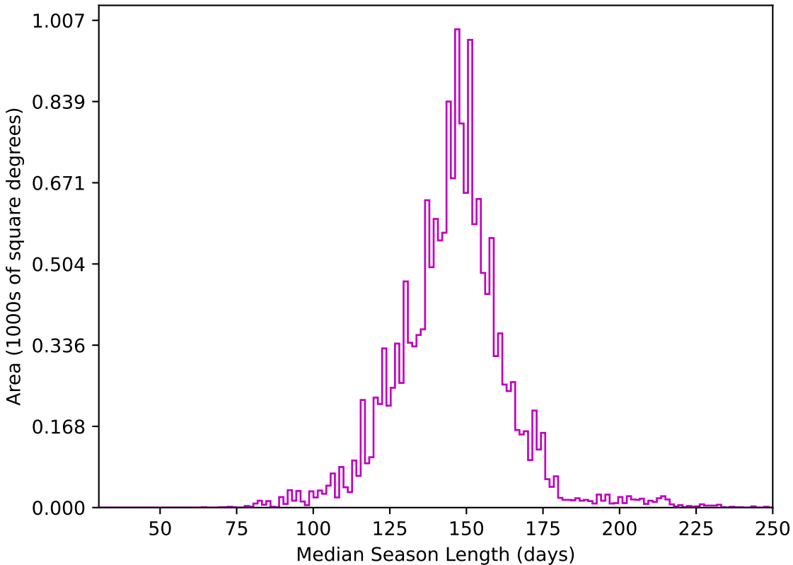
ddf_half_v3.4_10yrs WFD z band: Median Season Length
