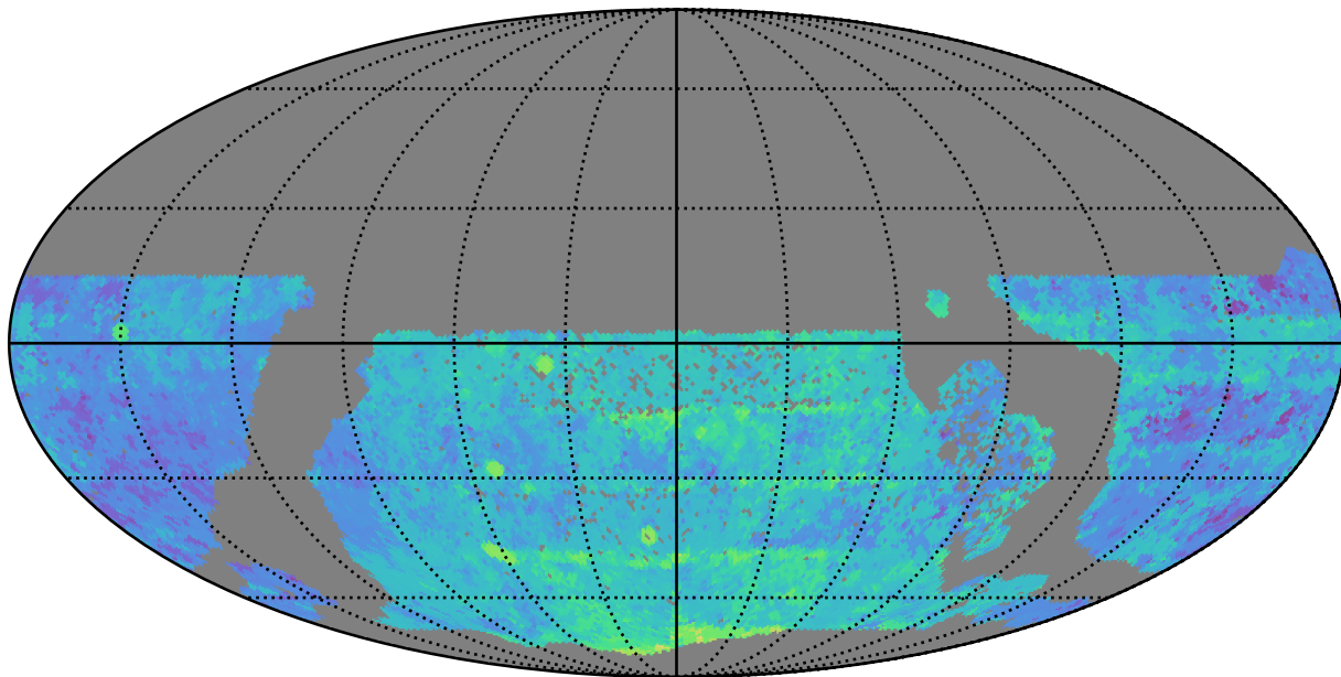
ddf_half_v3.4_10yrs WFD y band: Median Season Length
