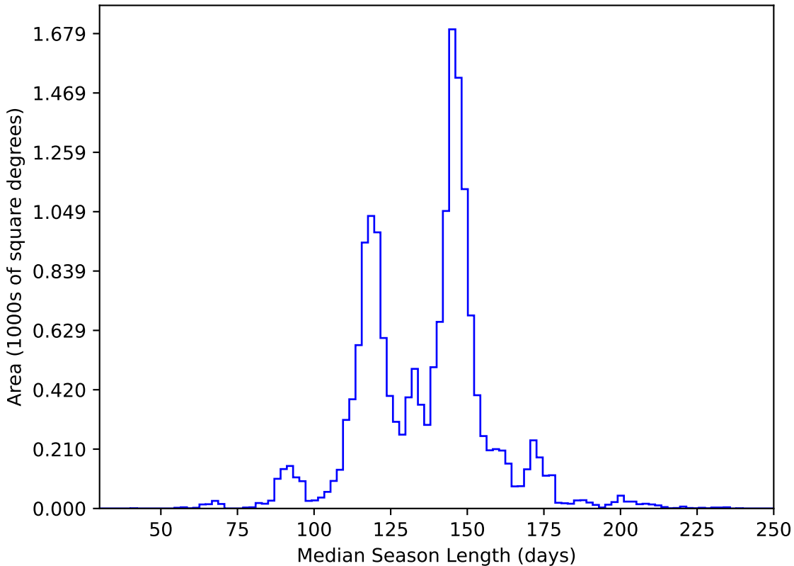
ddf_half_v3.4_10yrs WFD y band: Median Season Length
