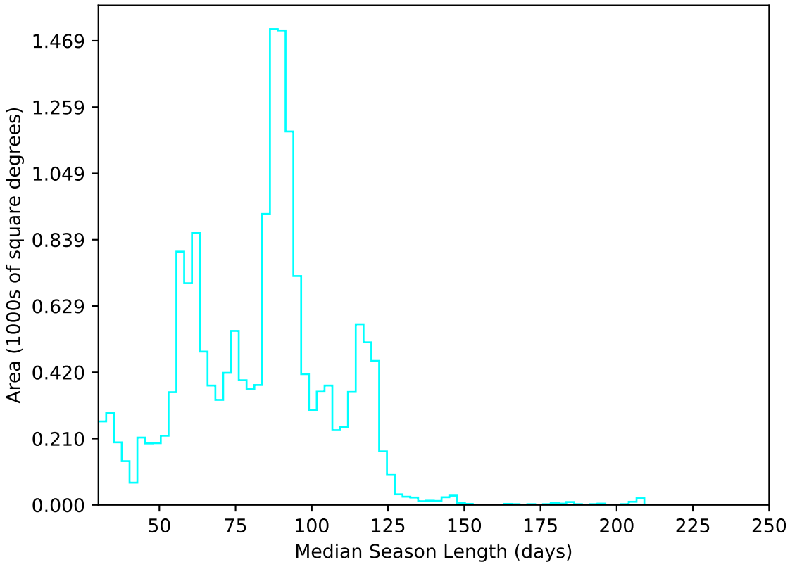
ddf_half_v3.4_10yrs WFD u band: Median Season Length
