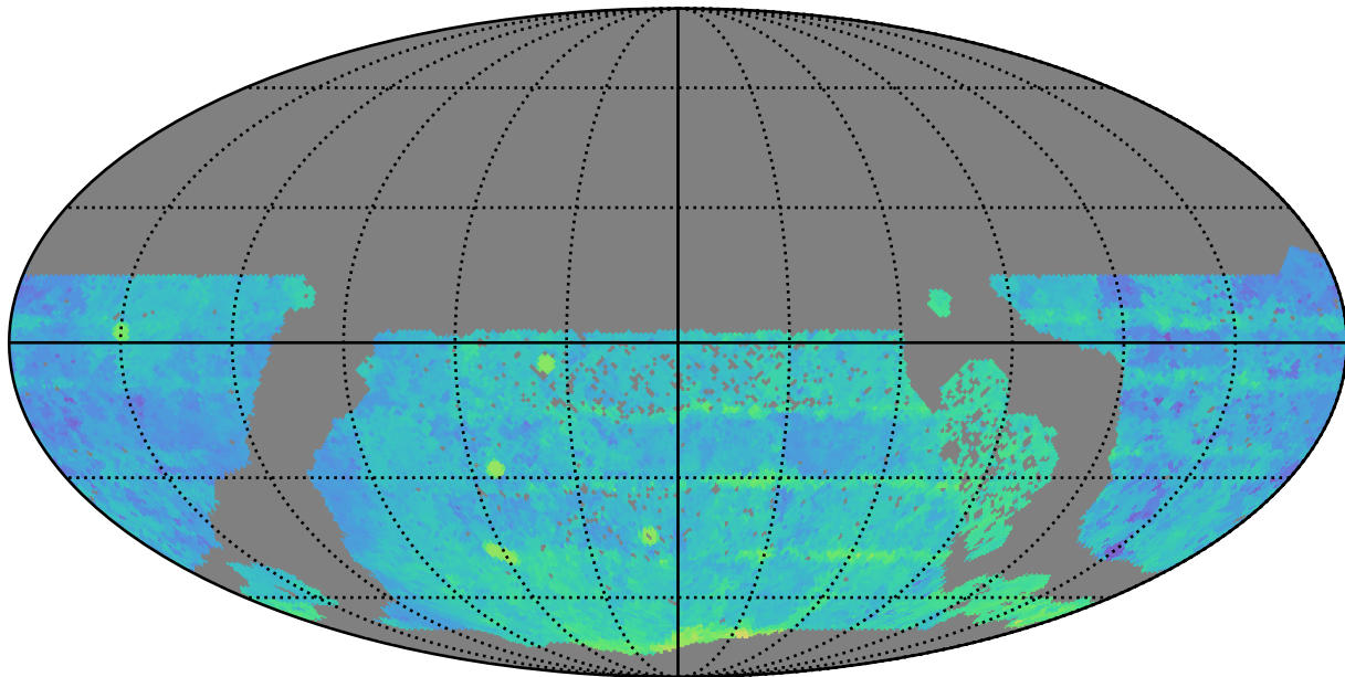
ddf_half_v3.4_10yrs WFD r band: Median Season Length
