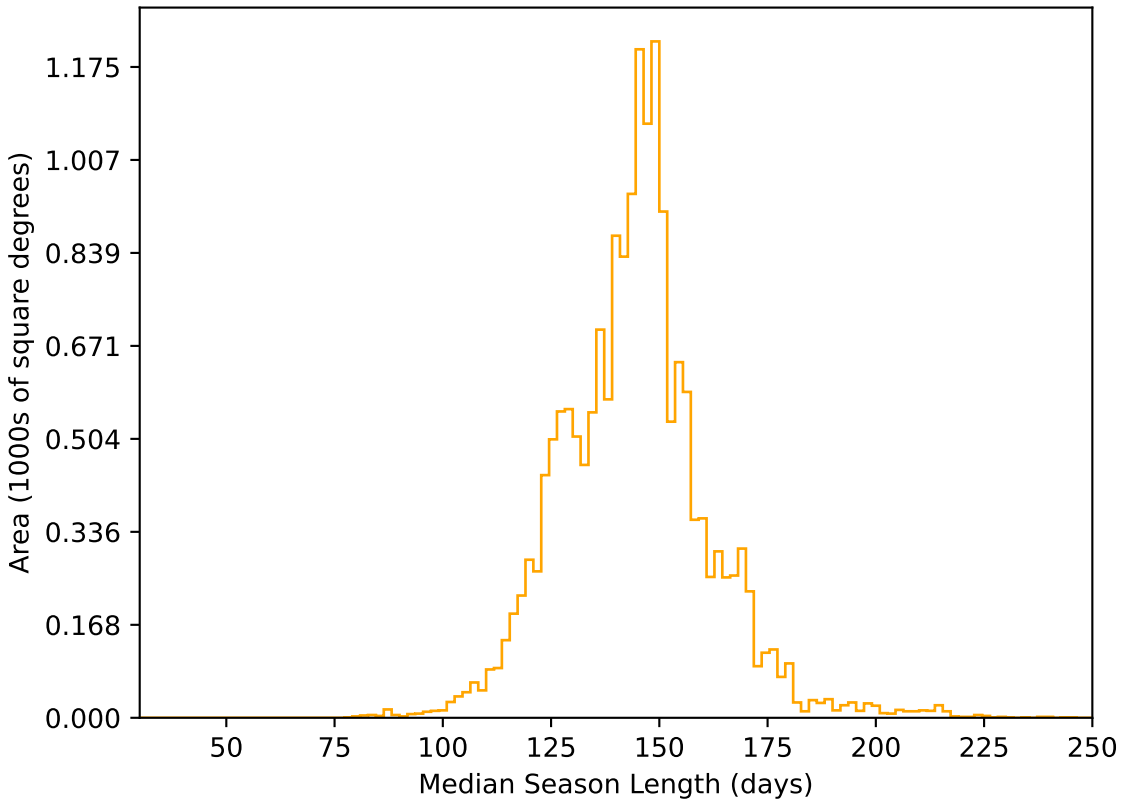
ddf_half_v3.4_10yrs WFD r band: Median Season Length
