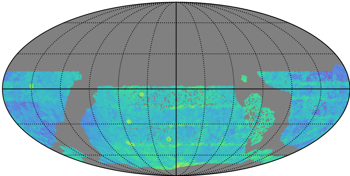
ddf_half_v3.4_10yrs WFD i band: Median Season Length
