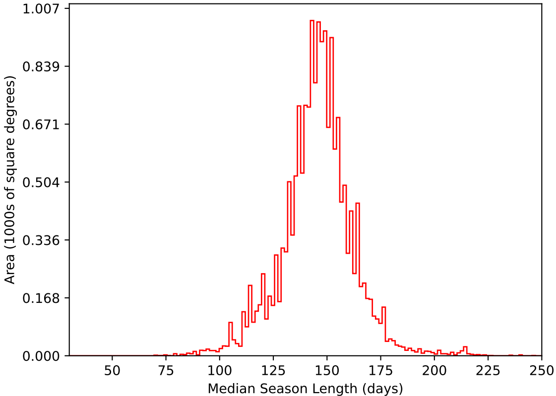
ddf_half_v3.4_10yrs WFD i band: Median Season Length
